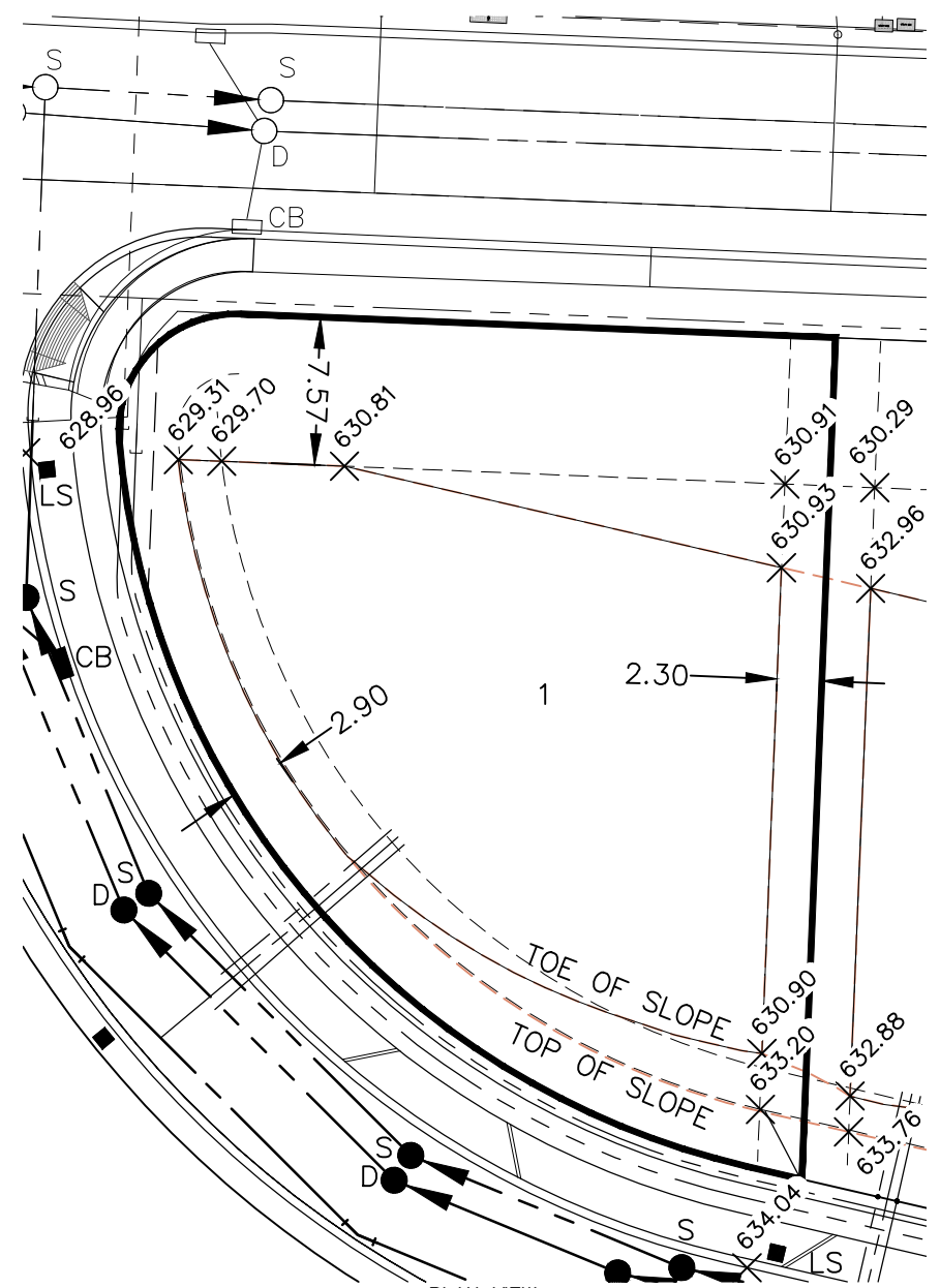
PLAN VIEW 1:400
