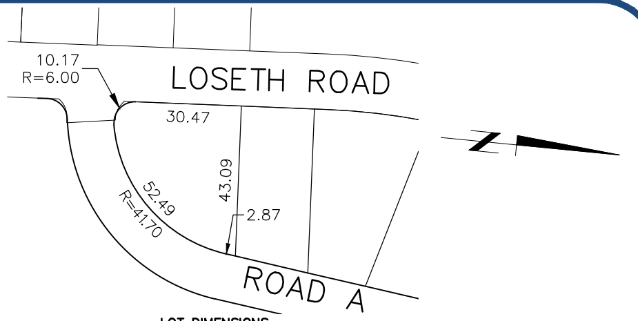
LOT DIMENSIONS 1:1500
