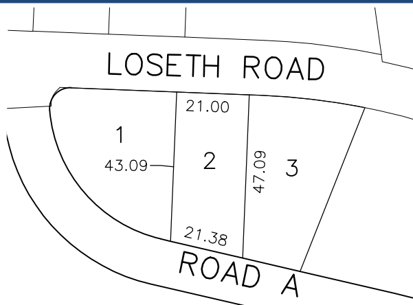
LOT DIMENSIONS 1:1500
